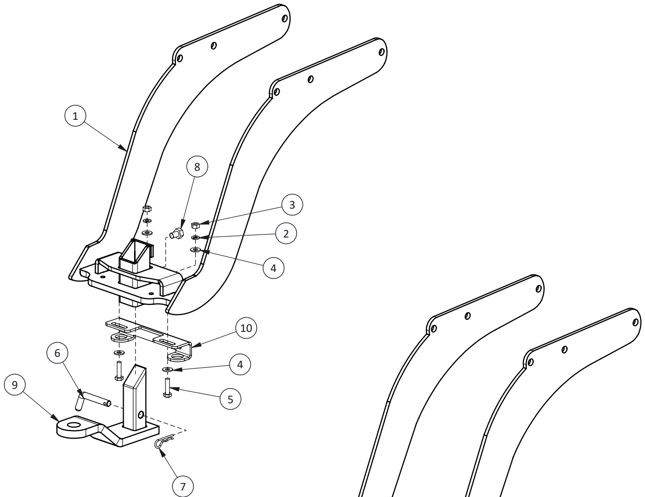
PARTIAL FRONT VIEW AT HITCH ASSEMBLY
