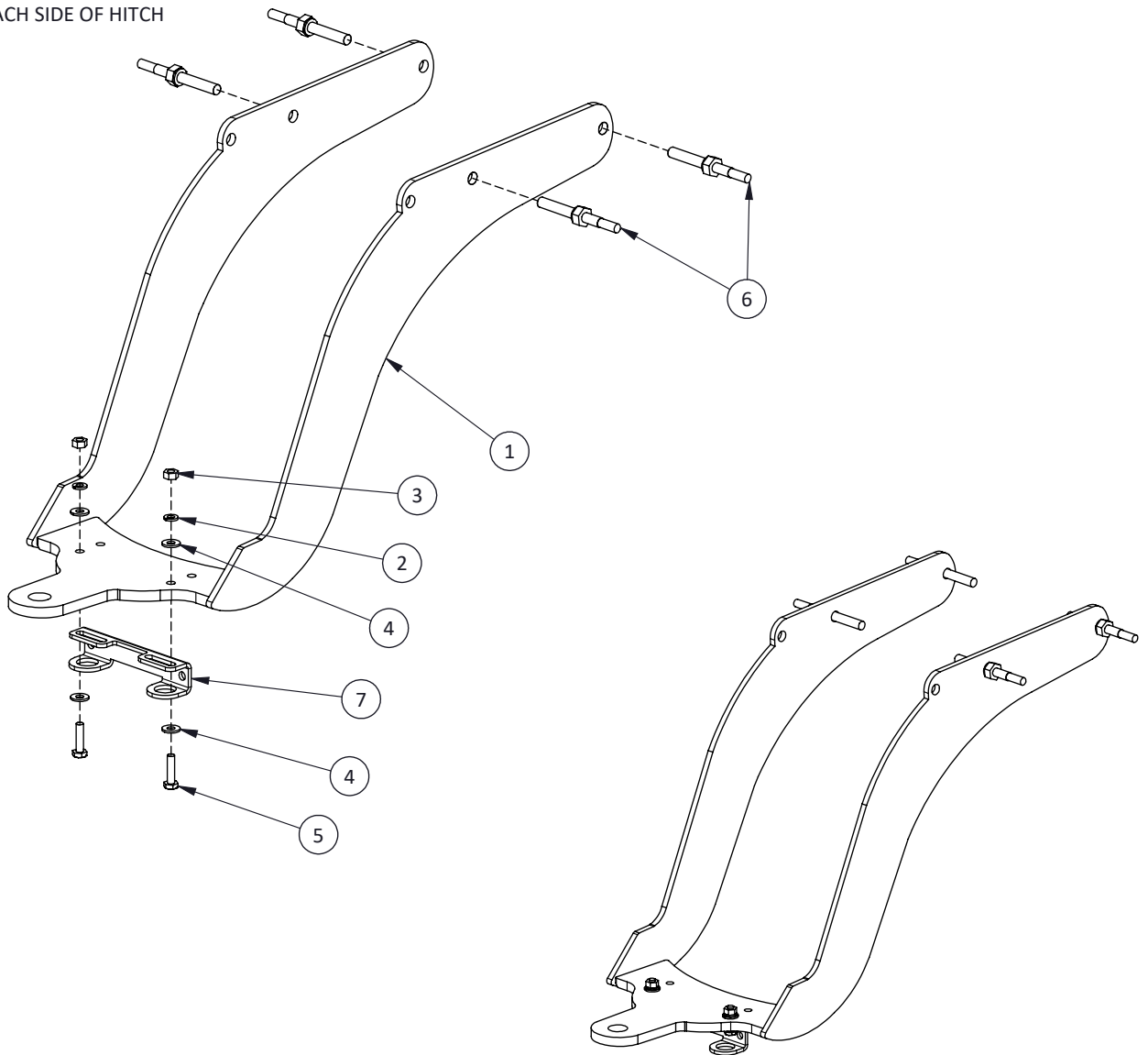
ASSEMBLED VIEW
