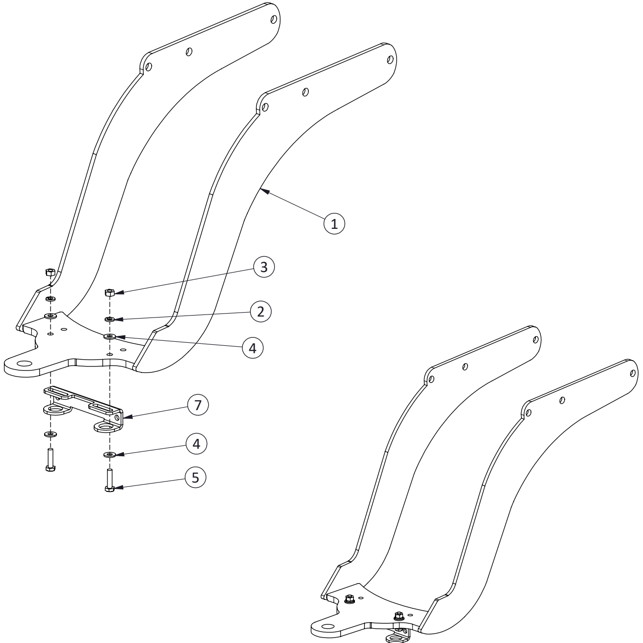
ASSEMBLED VIEW
