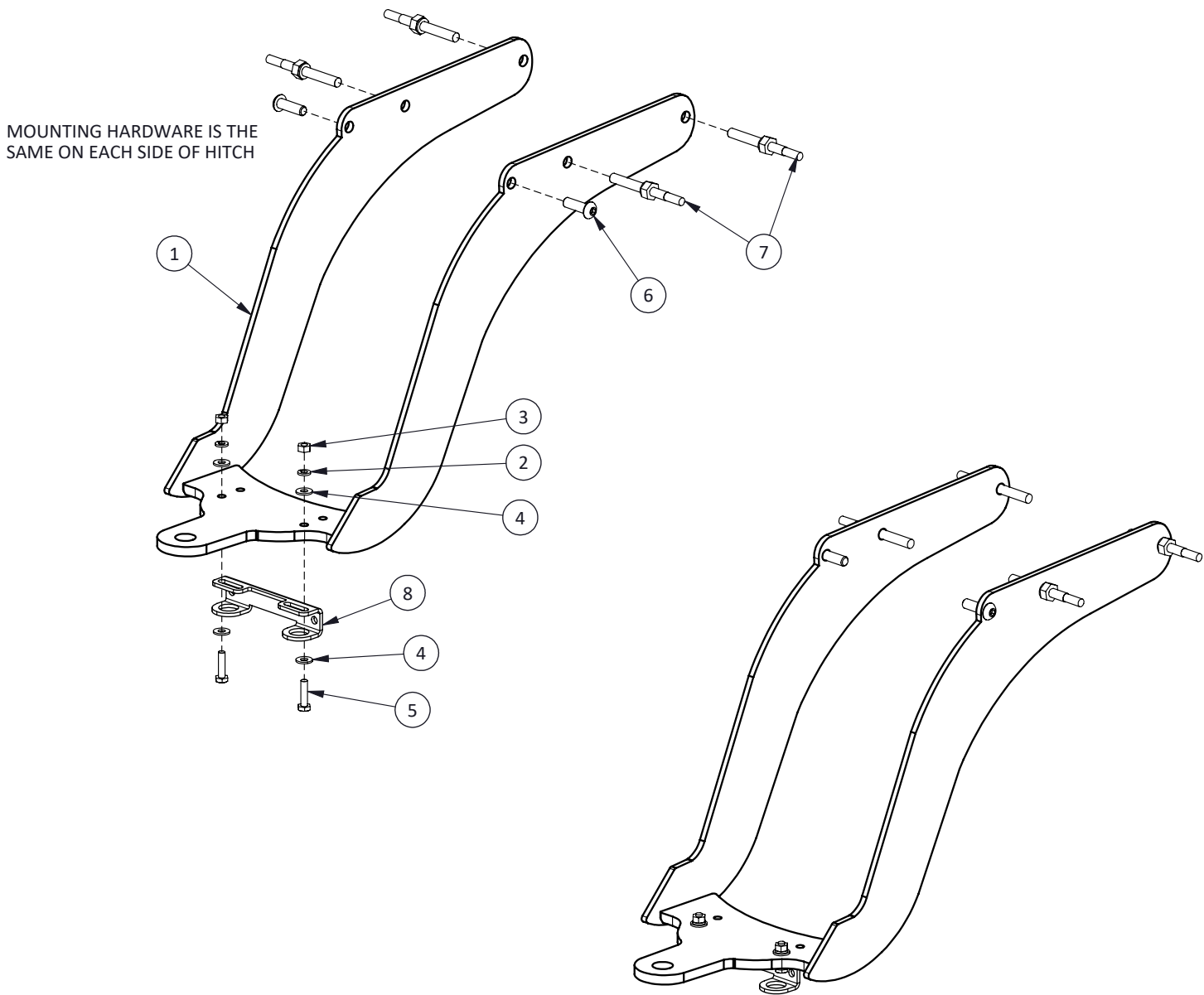
ASSEMBLED VIEW
