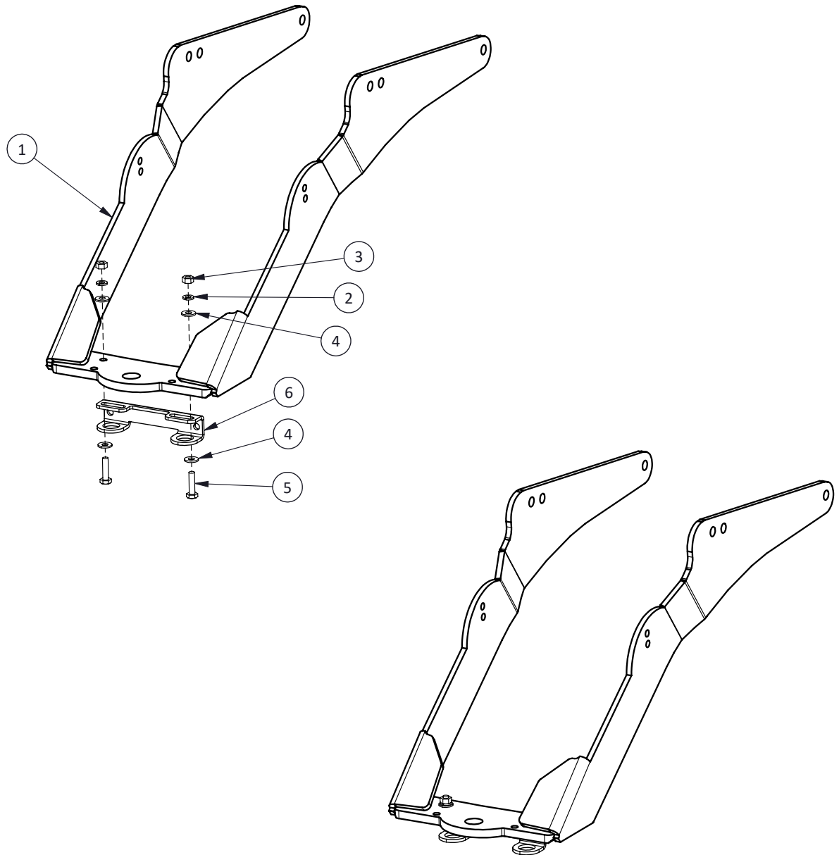
ASSEMBLED VIEW
