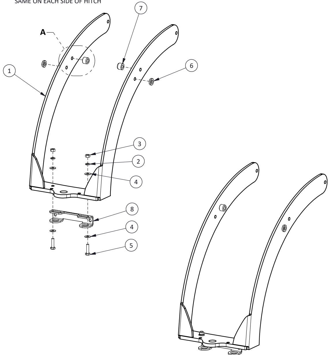
ASSEMBLED VIEW
